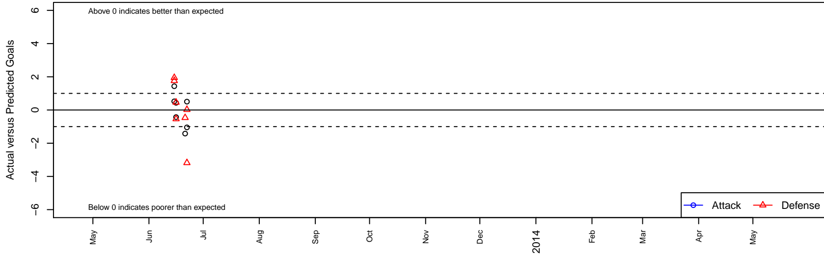
WSA Rapids Navy G01 Dots are actual minus expected GF (blue circles) and GA (red triangles). Blue line is smoothed change in attack strength. Red is smoothed change in defense strength.
